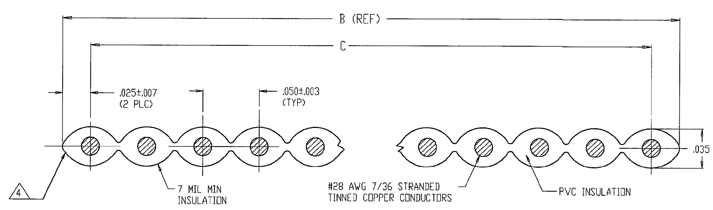
FLAT CABLE CROSS-SECTION
